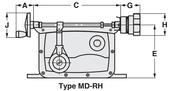
Microdial Control*
